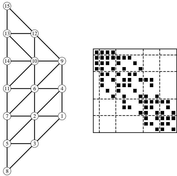
Figure 3.6 Cuthill-McKee ordering.
